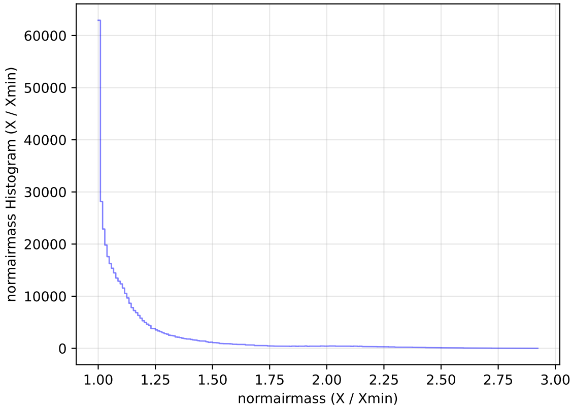
too_elab_r16_d3_griz_v3.4_10yrs WFD z band: normairmass Histogram
