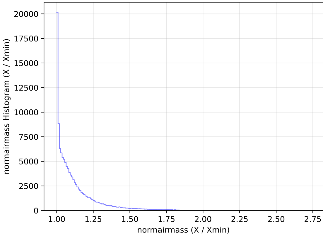
too_elab_r16_d3_griz_v3.4_10yrs WFD u band: normairmass Histogram
