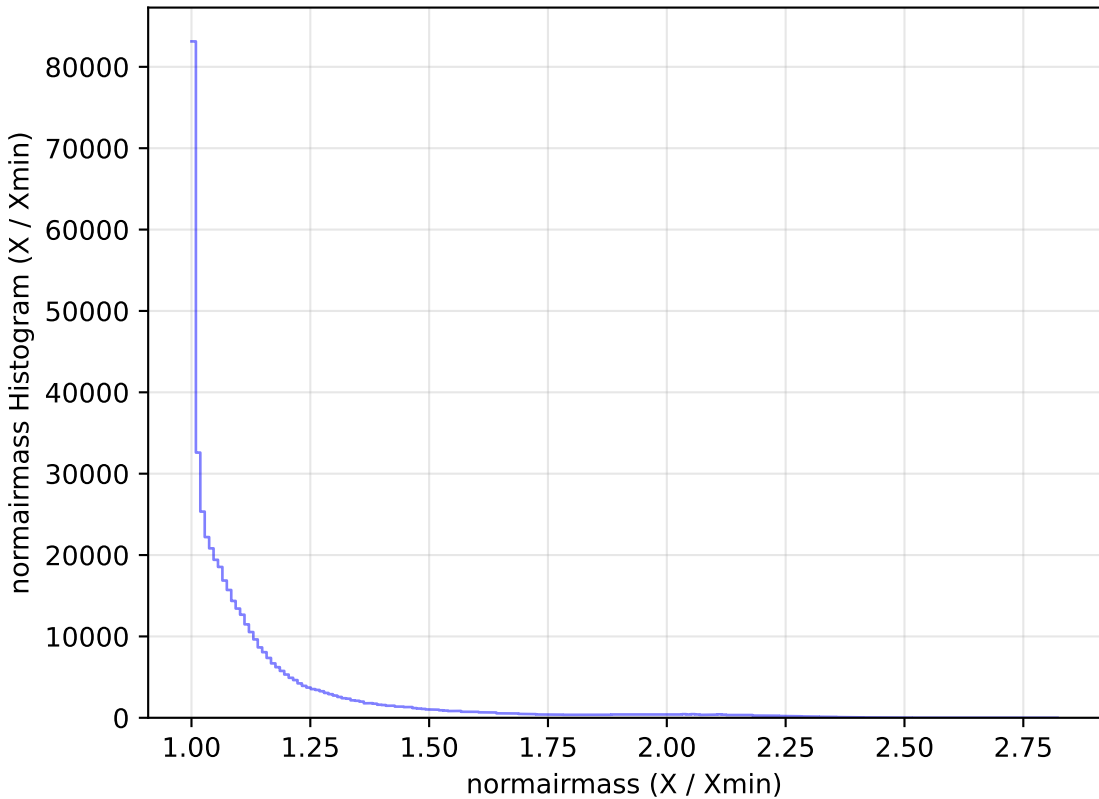
too_elab_r16_d3_griz_v3.4_10yrs WFD r band: normairmass Histogram
