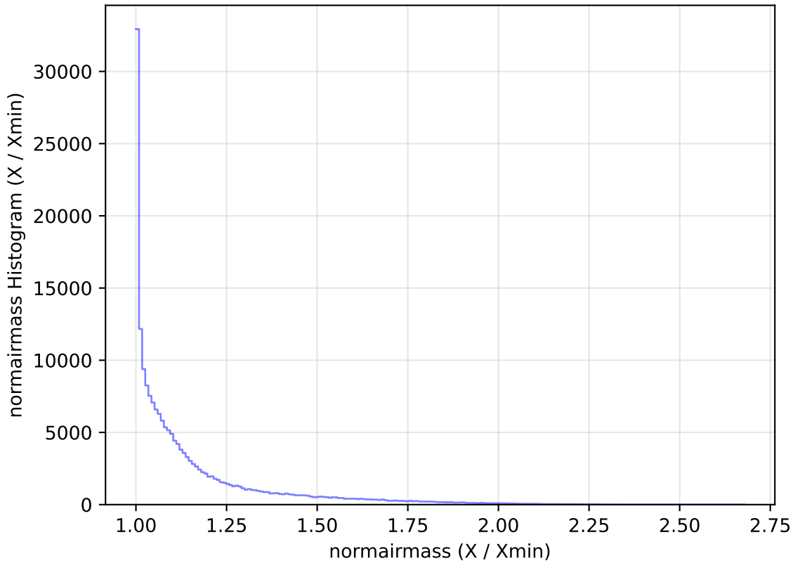
too_elab_r16_d3_griz_v3.4_10yrs WFD g band: normairmass Histogram
