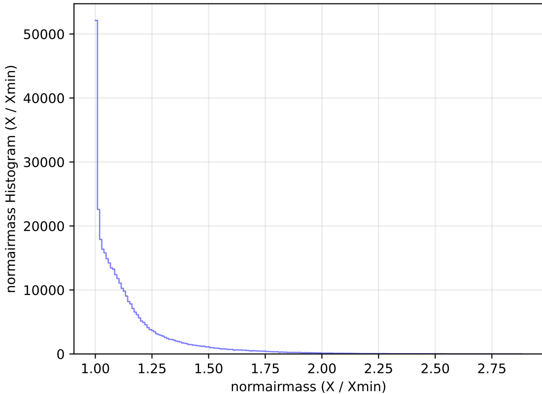
too_elab_r16_d3_griz_v3.4_10yrs All sky y band: normairmass Histogram
