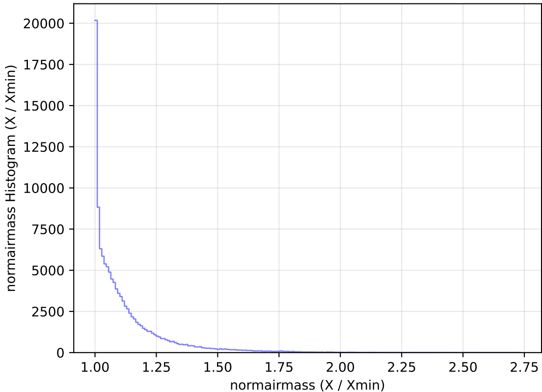
too_elab_r16_d3_griz_v3.4_10yrs All sky u band: normairmass Histogram
