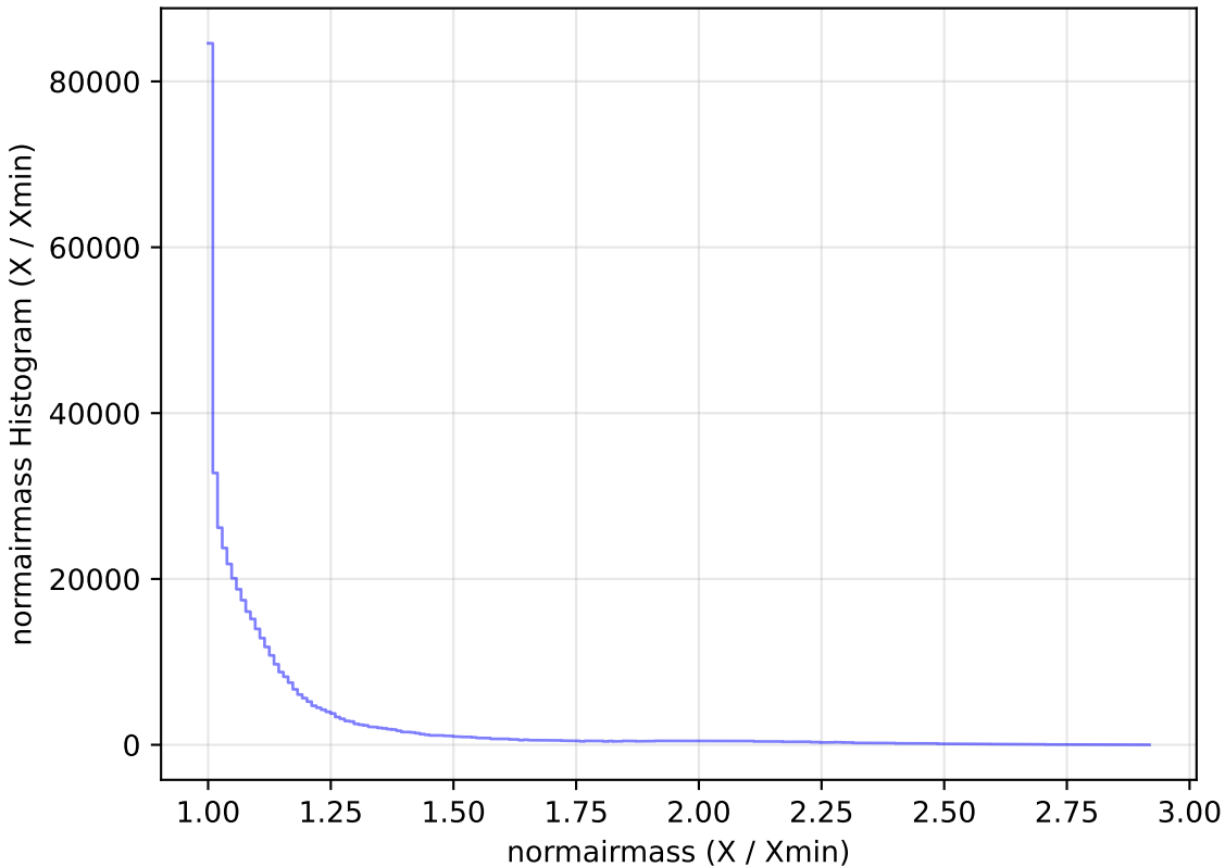
too_elab_r16_d3_griz_v3.4_10yrs All sky i band: normairmass Histogram
