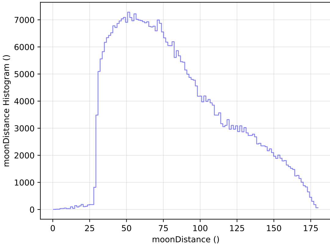
too_elab_r16_d3_griz_v3.4_10yrs WFD z band: moonDistance Histogram
