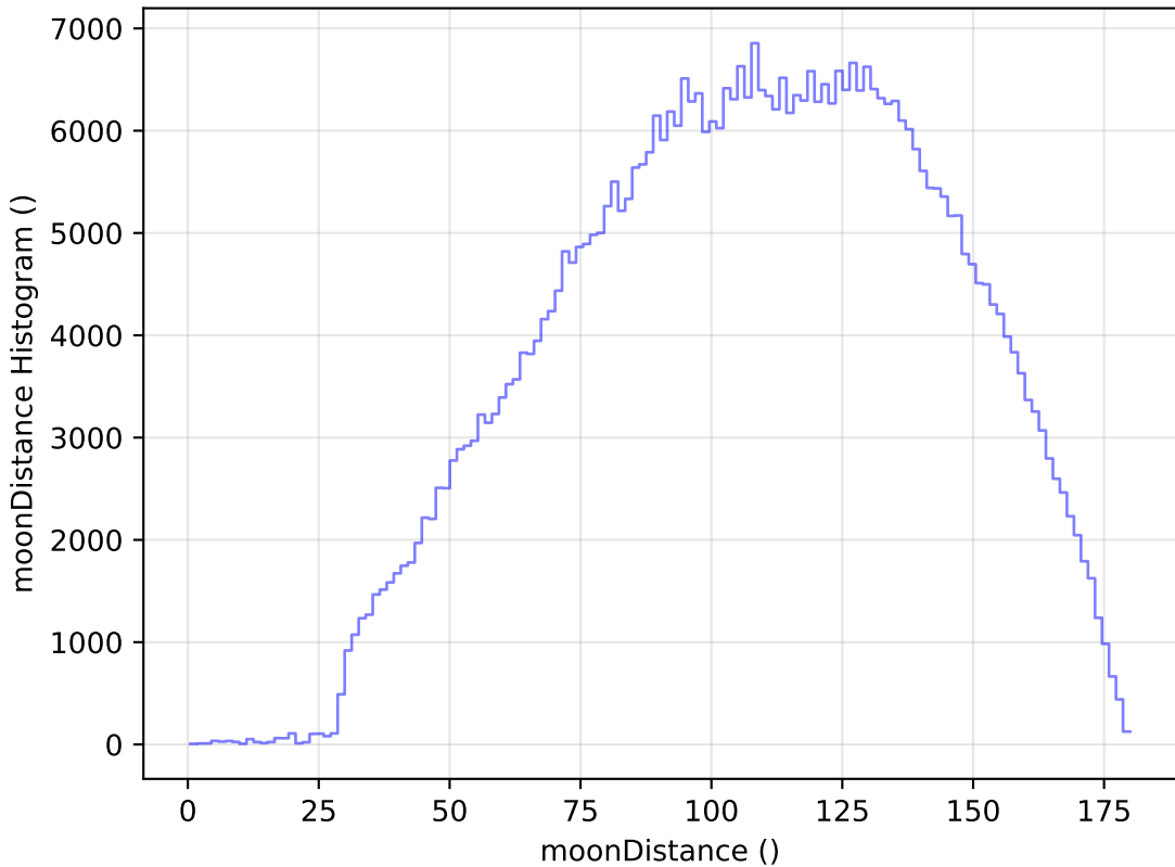
too_elab_r16_d3_griz_v3.4_10yrs WFD r band: moonDistance Histogram
