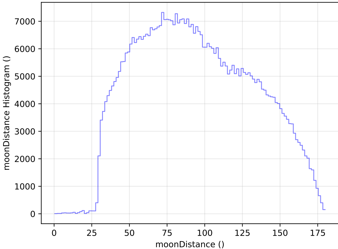
too_elab_r16_d3_griz_v3.4_10yrs WFD i band: moonDistance Histogram
