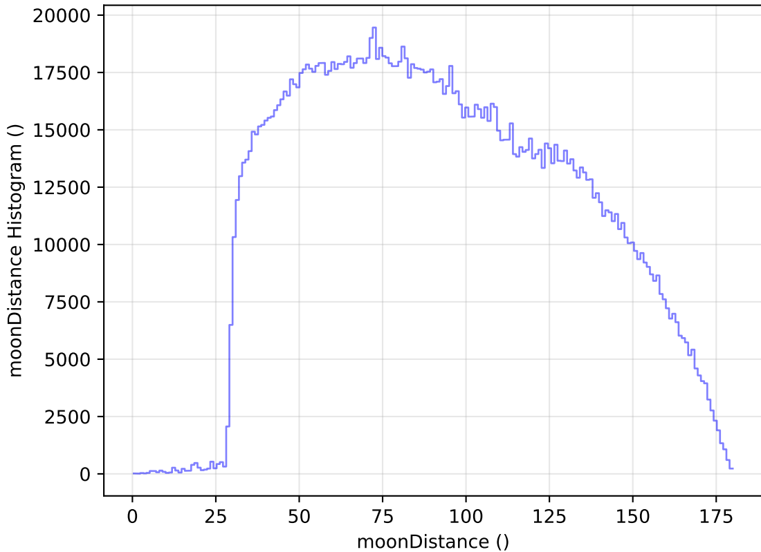
too_elab_r16_d3_griz_v3.4_10yrs WFD all bands: moonDistance Histogram
