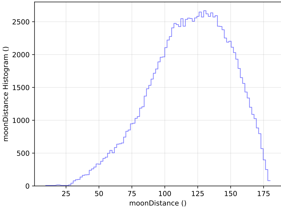
too_elab_r16_d3_griz_v3.4_10yrs All sky u band: moonDistance Histogram
