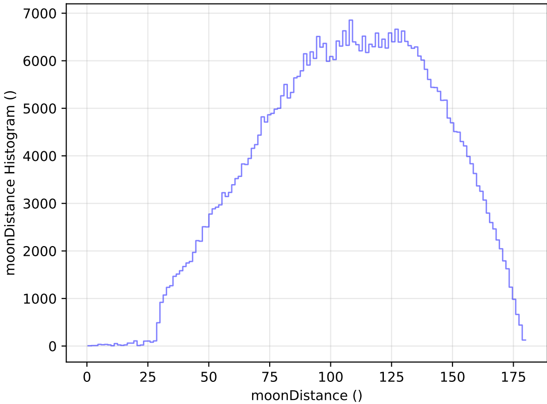
too_elab_r16_d3_griz_v3.4_10yrs All sky r band: moonDistance Histogram
