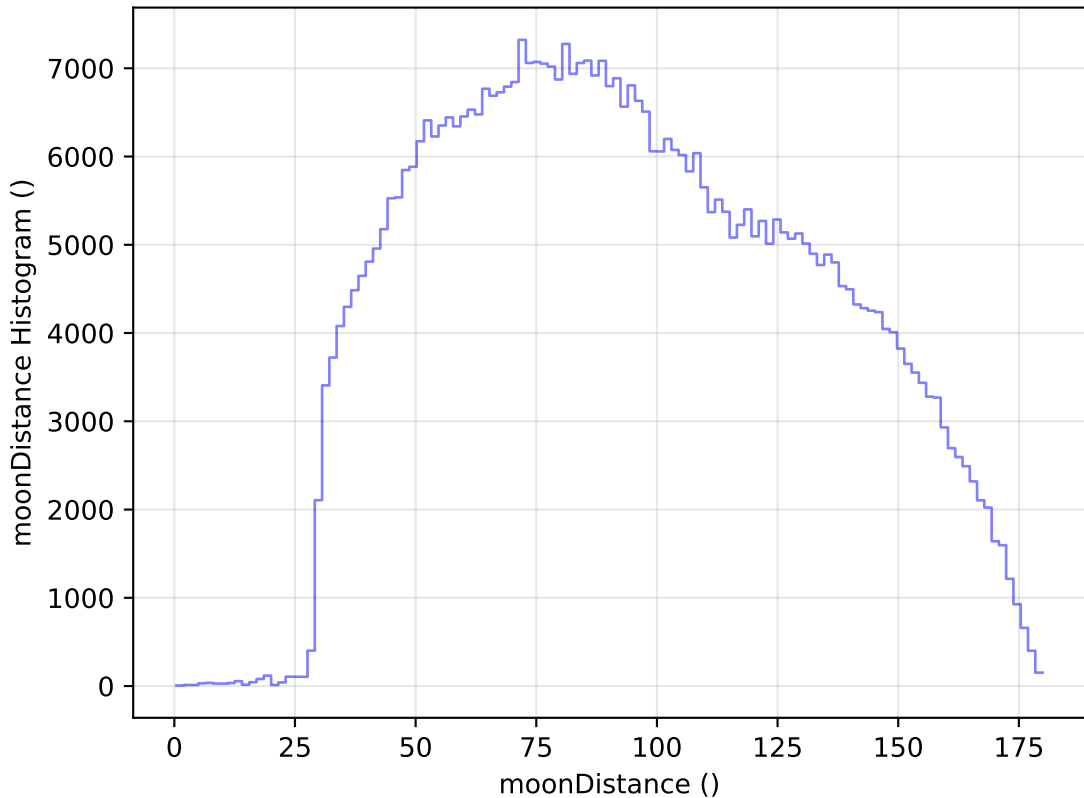
too_elab_r16_d3_griz_v3.4_10yrs All sky i band: moonDistance Histogram
