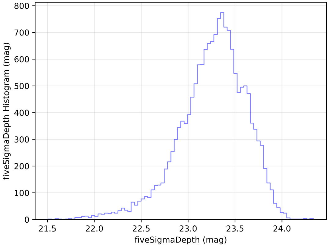
too_elab_r16_d3_griz_v3.4_10yrs Yr 1 u band: fiveSigmaDepth Histogram
