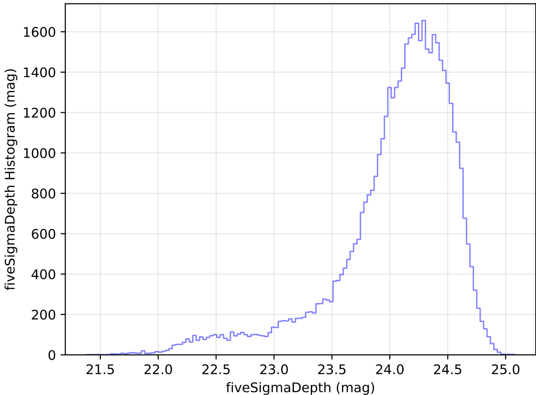
too_elab_r16_d3_griz_v3.4_10yrs Yr 1 r band: fiveSigmaDepth Histogram
