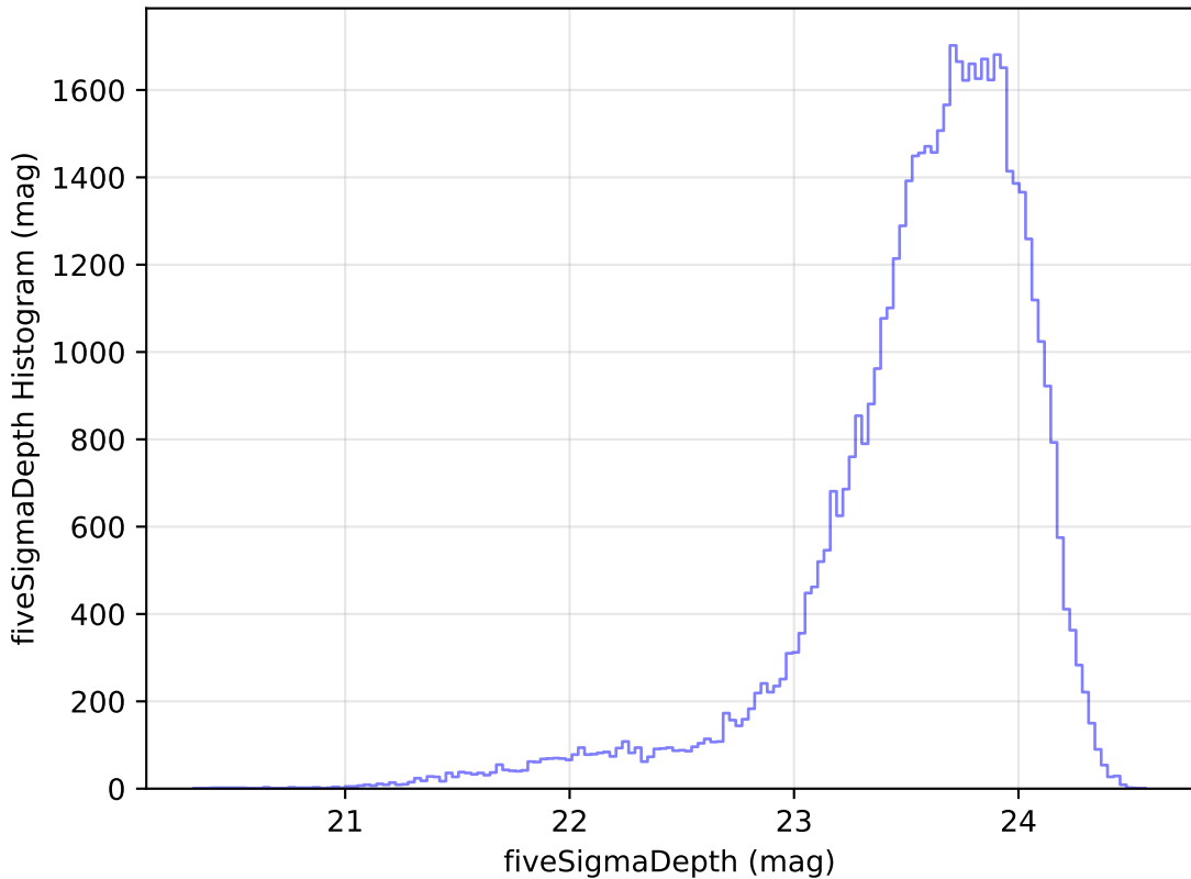
too_elab_r16_d3_griz_v3.4_10yrs Yr 1 i band: fiveSigmaDepth Histogram
