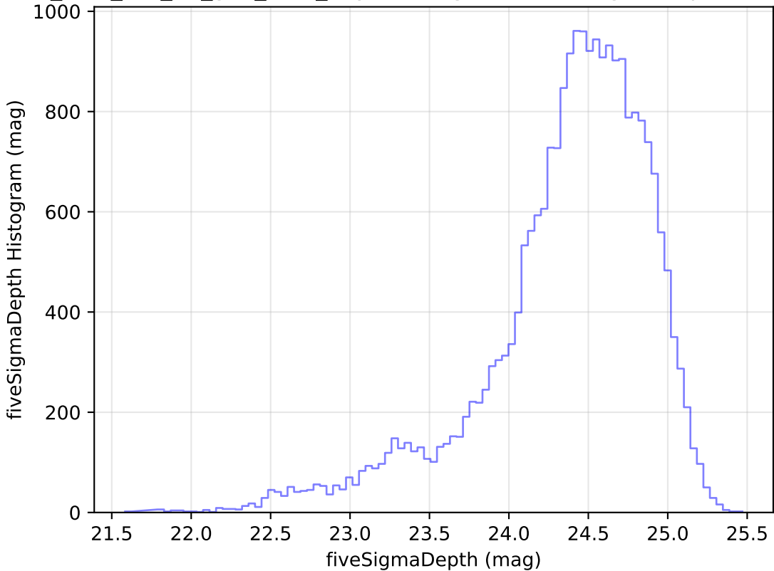
too_elab_r16_d3_griz_v3.4_10yrs Yr 1 g band: fiveSigmaDepth Histogram
