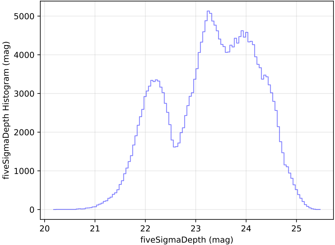
too_elab_r16_d3_griz_v3.4_10yrs Yr 1 all bands: fiveSigmaDepth Histogram
