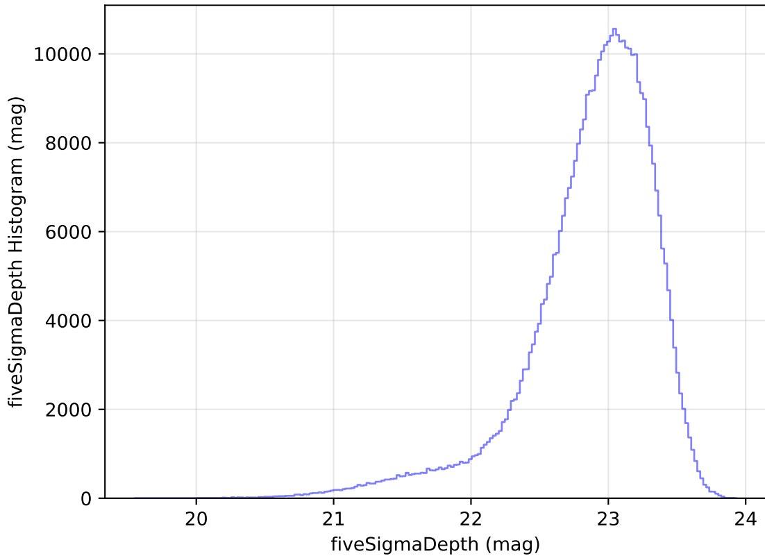
too_elab_r16_d3_griz_v3.4_10yrs WFD z band: fiveSigmaDepth Histogram
