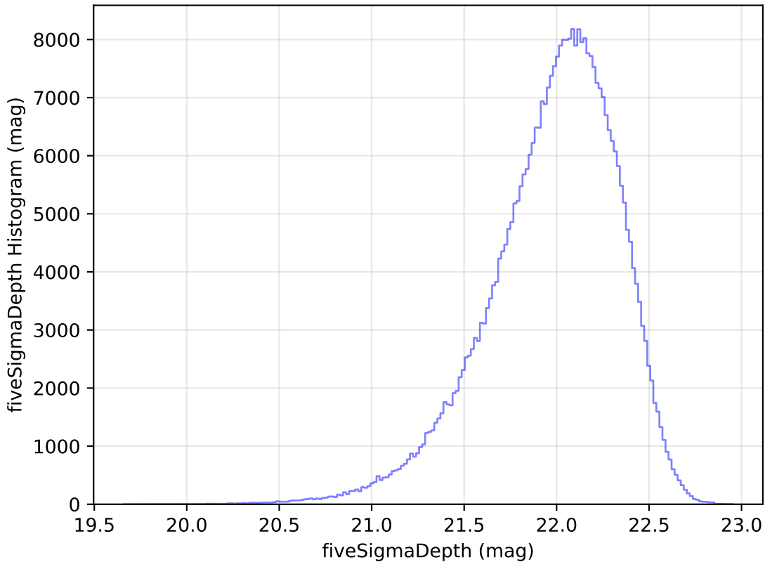
too_elab_r16_d3_griz_v3.4_10yrs WFD y band: fiveSigmaDepth Histogram
