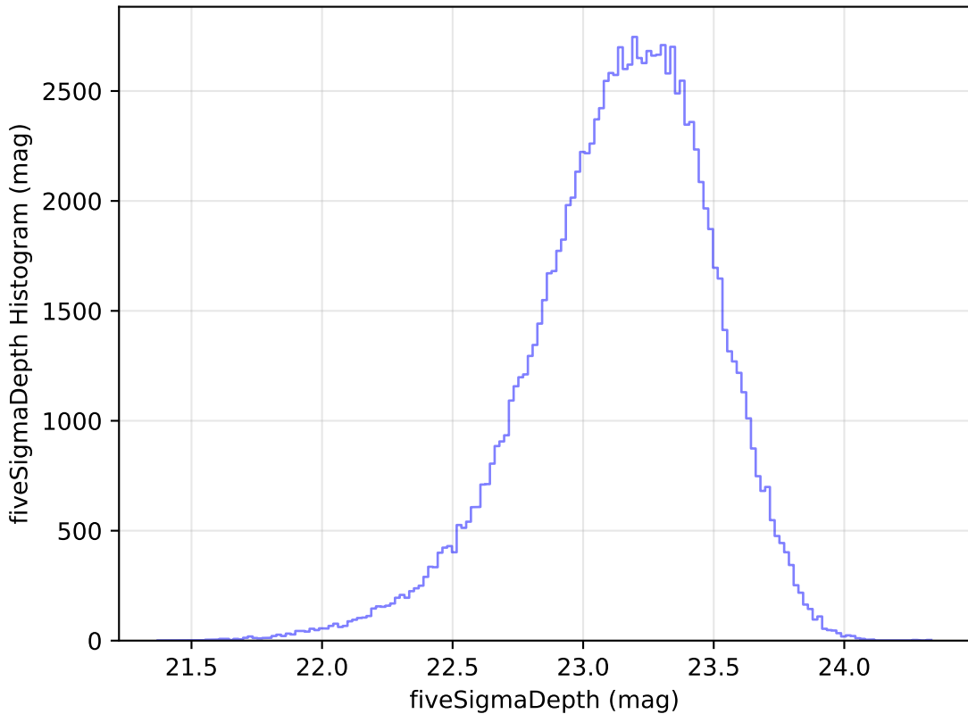
too_elab_r16_d3_griz_v3.4_10yrs WFD u band: fiveSigmaDepth Histogram
