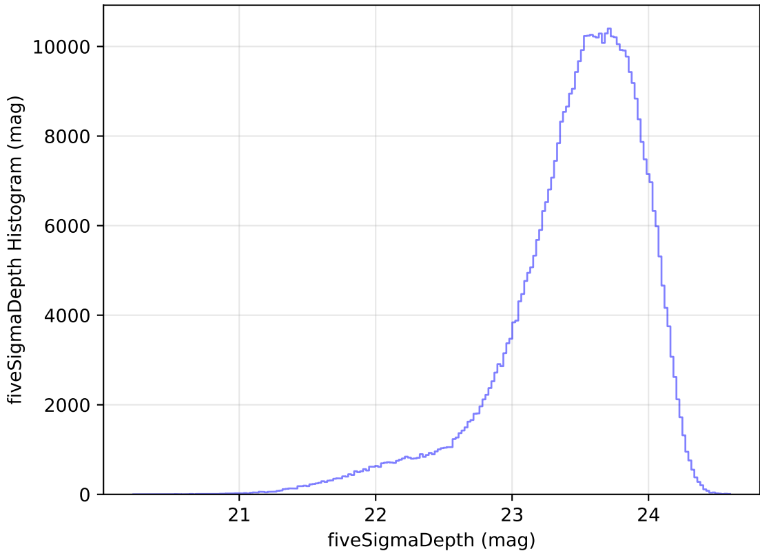
too_elab_r16_d3_griz_v3.4_10yrs WFD i band: fiveSigmaDepth Histogram
