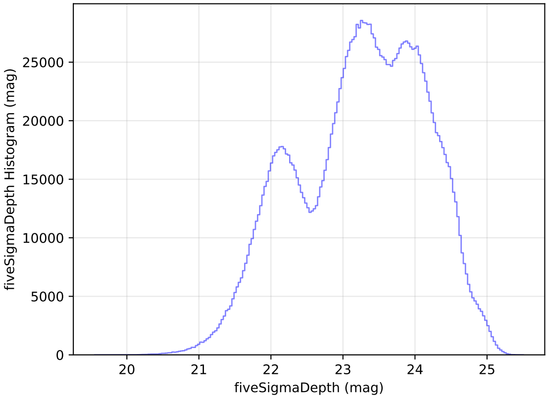
too_elab_r16_d3_griz_v3.4_10yrs WFD all bands: fiveSigmaDepth Histogram
