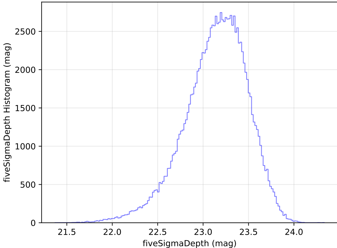
too_elab_r16_d3_griz_v3.4_10yrs All sky u band: fiveSigmaDepth Histogram
