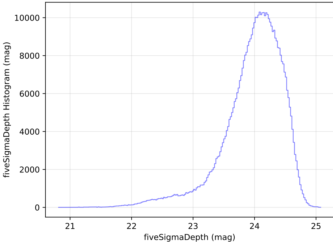
too_elab_r16_d3_griz_v3.4_10yrs All sky r band: fiveSigmaDepth Histogram
