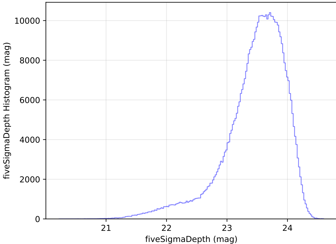
too_elab_r16_d3_griz_v3.4_10yrs All sky i band: fiveSigmaDepth Histogram
