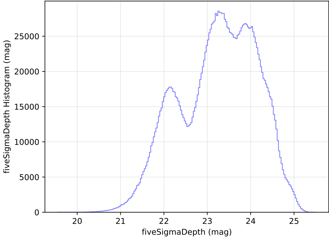
too_elab_r16_d3_griz_v3.4_10yrs All sky all bands: fiveSigmaDepth Histogram
