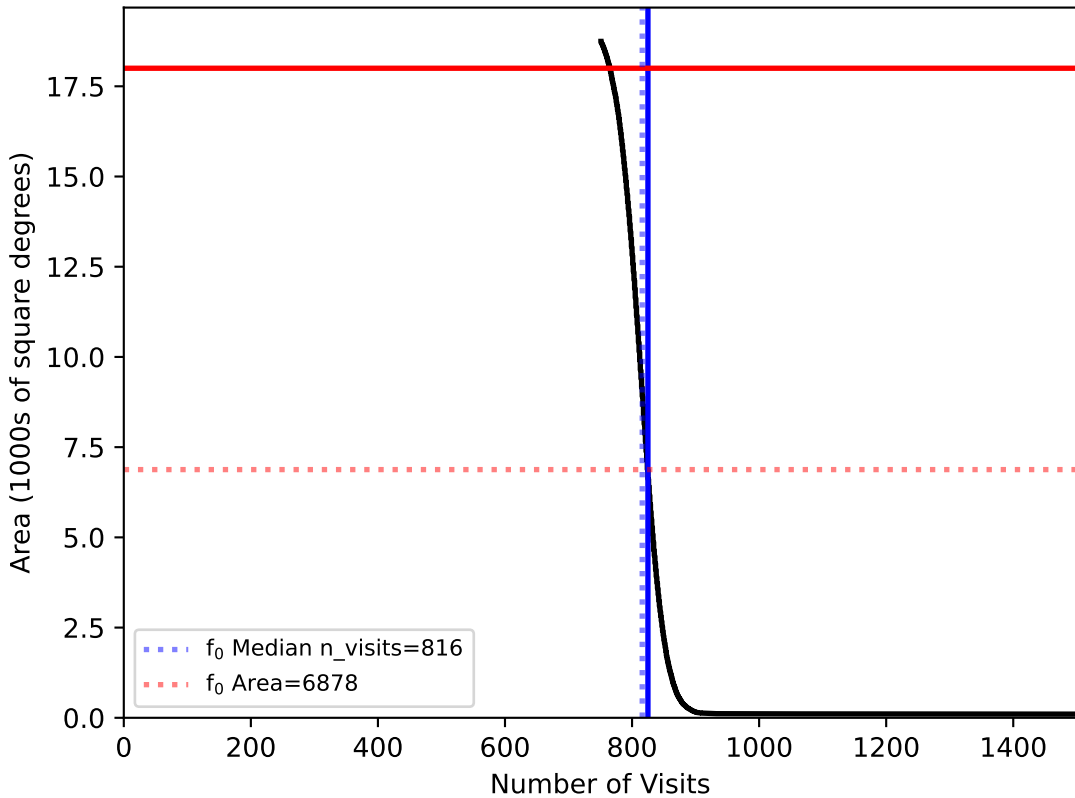
too_elab_r16_d3_griz_v3.4_10yrs WFD: fO
