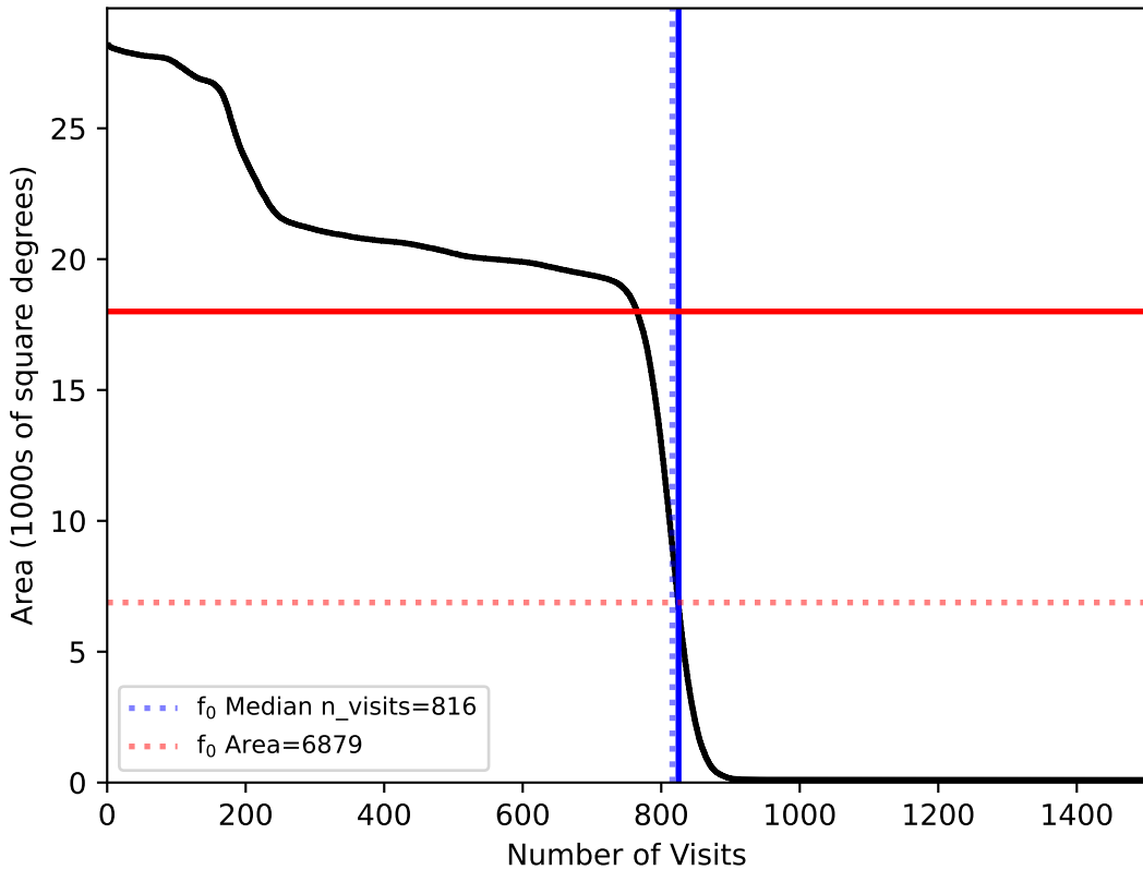
too_elab_r16_d3_griz_v3.4_10yrs All sky: fO
