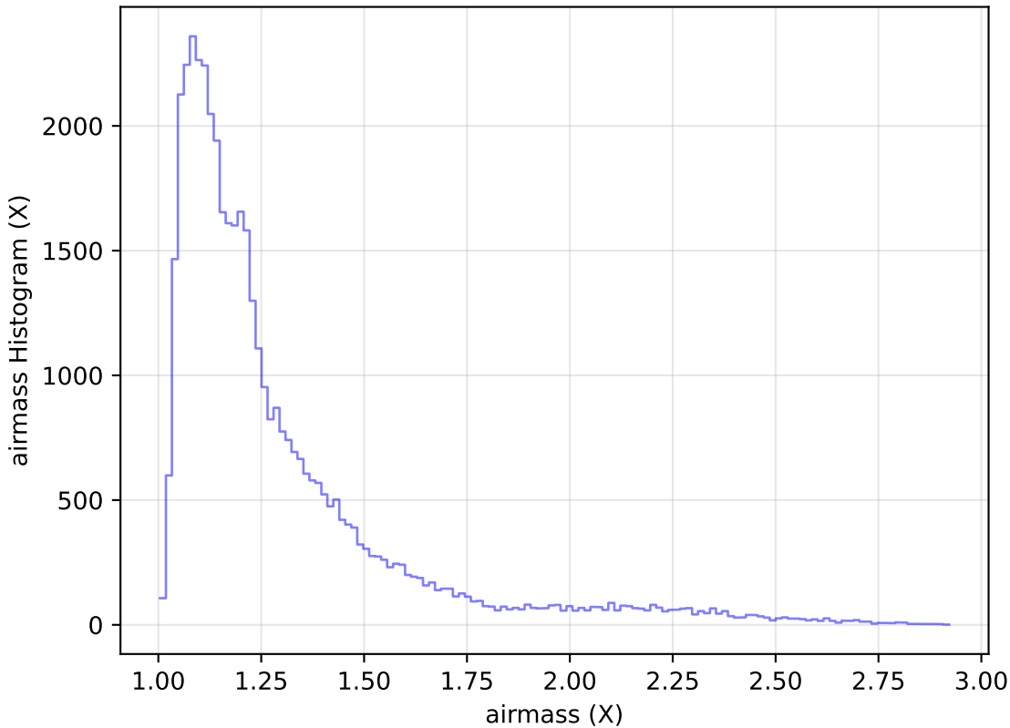
too_elab_r16_d3_griz_v3.4_10yrs Yr 1 z band: airmass Histogram
