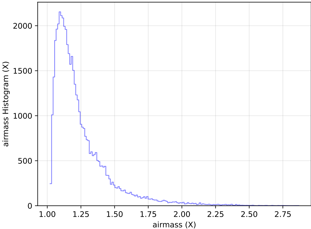
too_elab_r16_d3_griz_v3.4_10yrs Yr 1 y band: airmass Histogram
