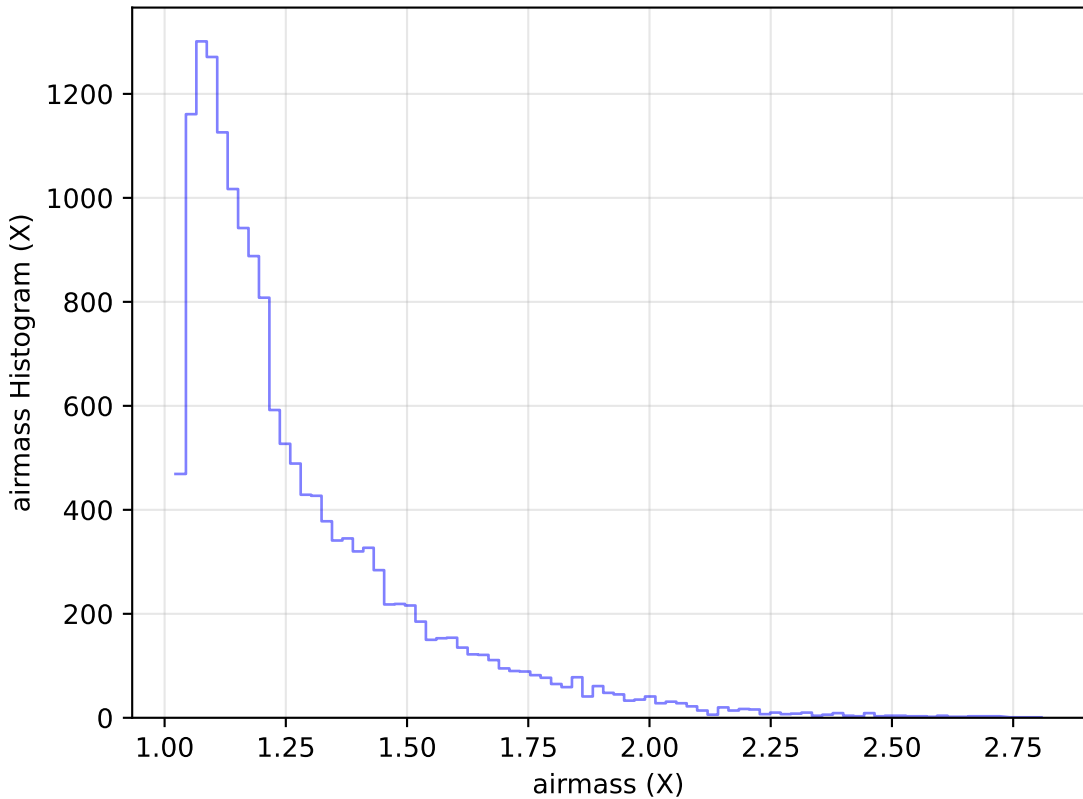
too_elab_r16_d3_griz_v3.4_10yrs Yr 1 u band: airmass Histogram
