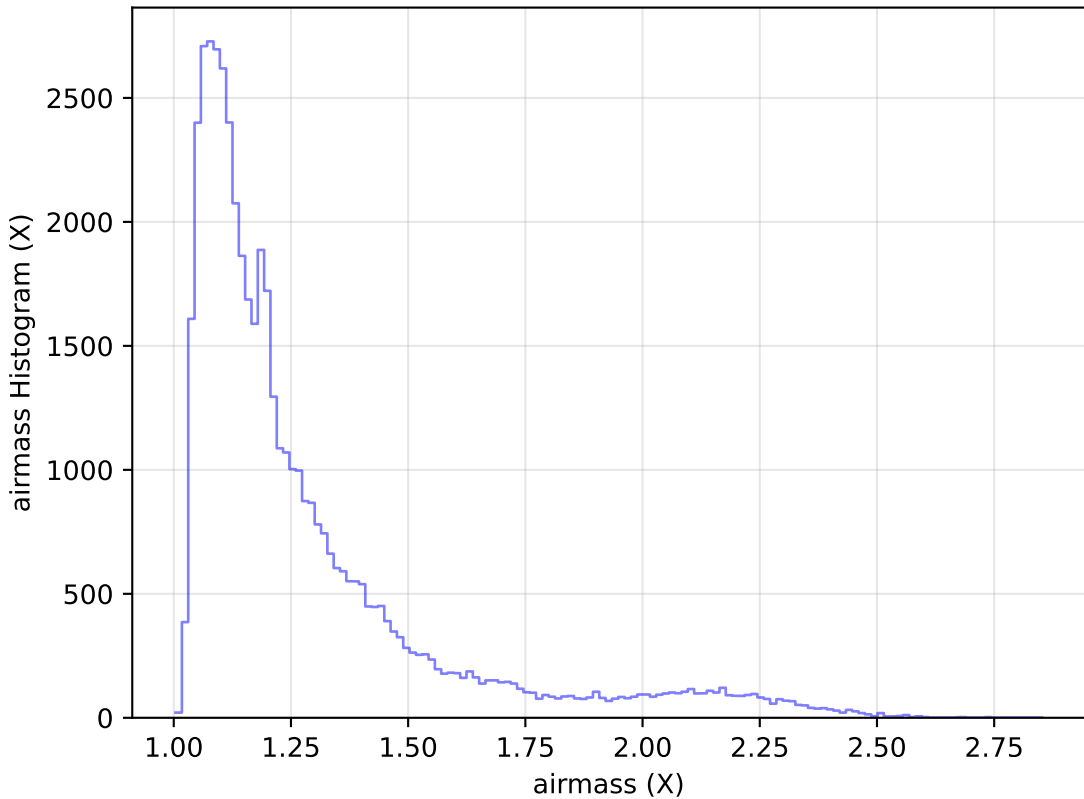
too_elab_r16_d3_griz_v3.4_10yrs Yr 1 r band: airmass Histogram
