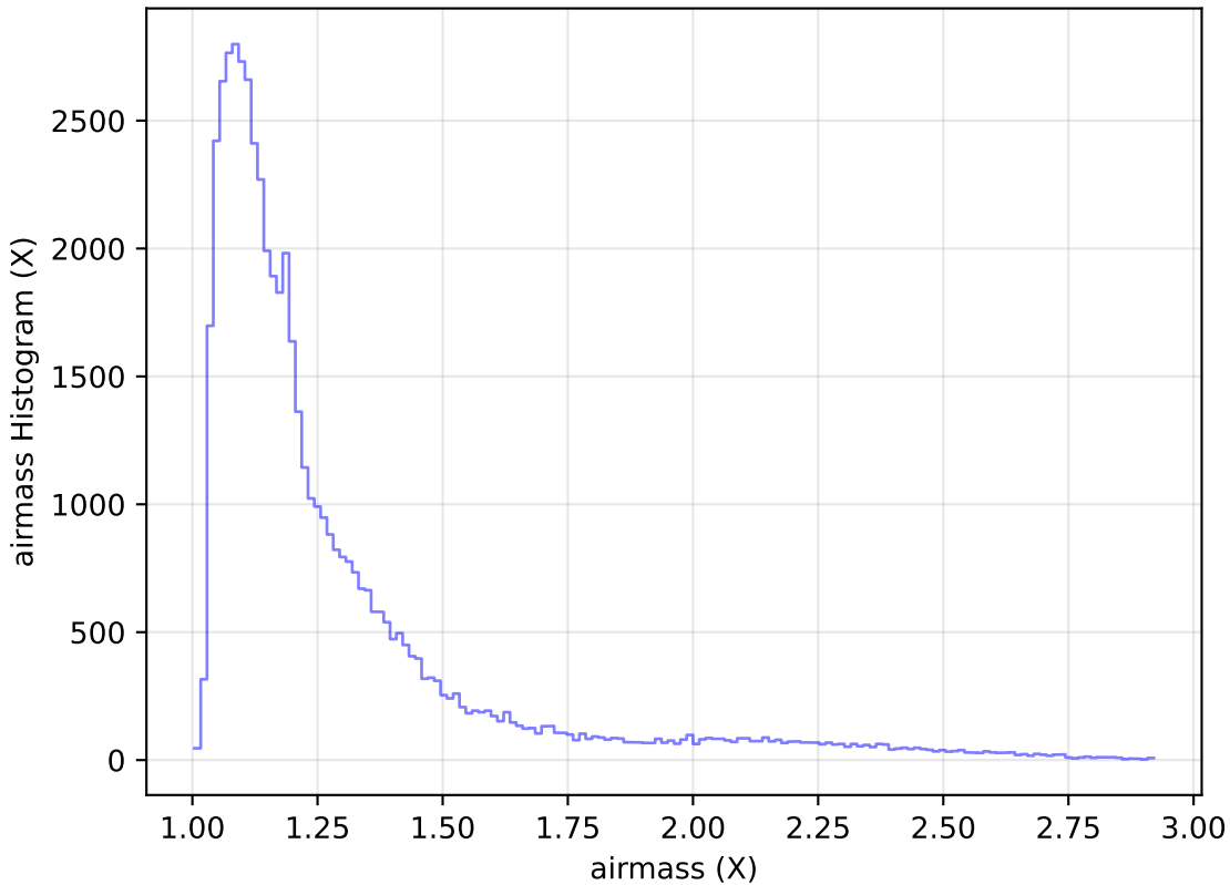
too_elab_r16_d3_griz_v3.4_10yrs Yr 1 i band: airmass Histogram
