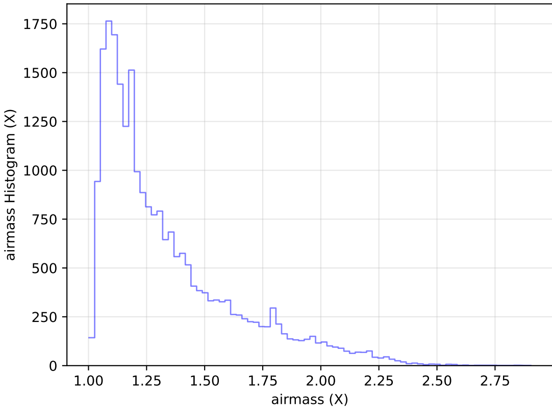
too_elab_r16_d3_griz_v3.4_10yrs Yr 1 g band: airmass Histogram
