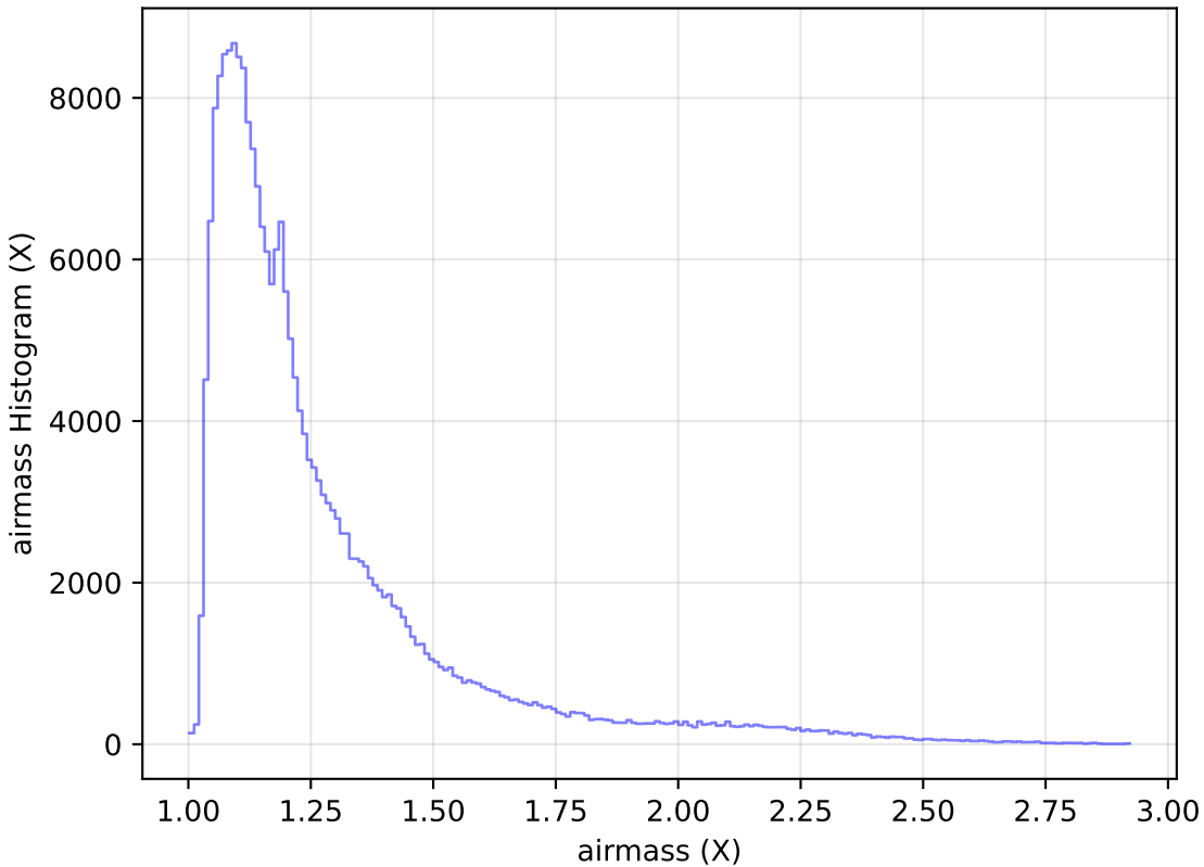
too_elab_r16_d3_griz_v3.4_10yrs Yr 1 all bands: airmass Histogram
