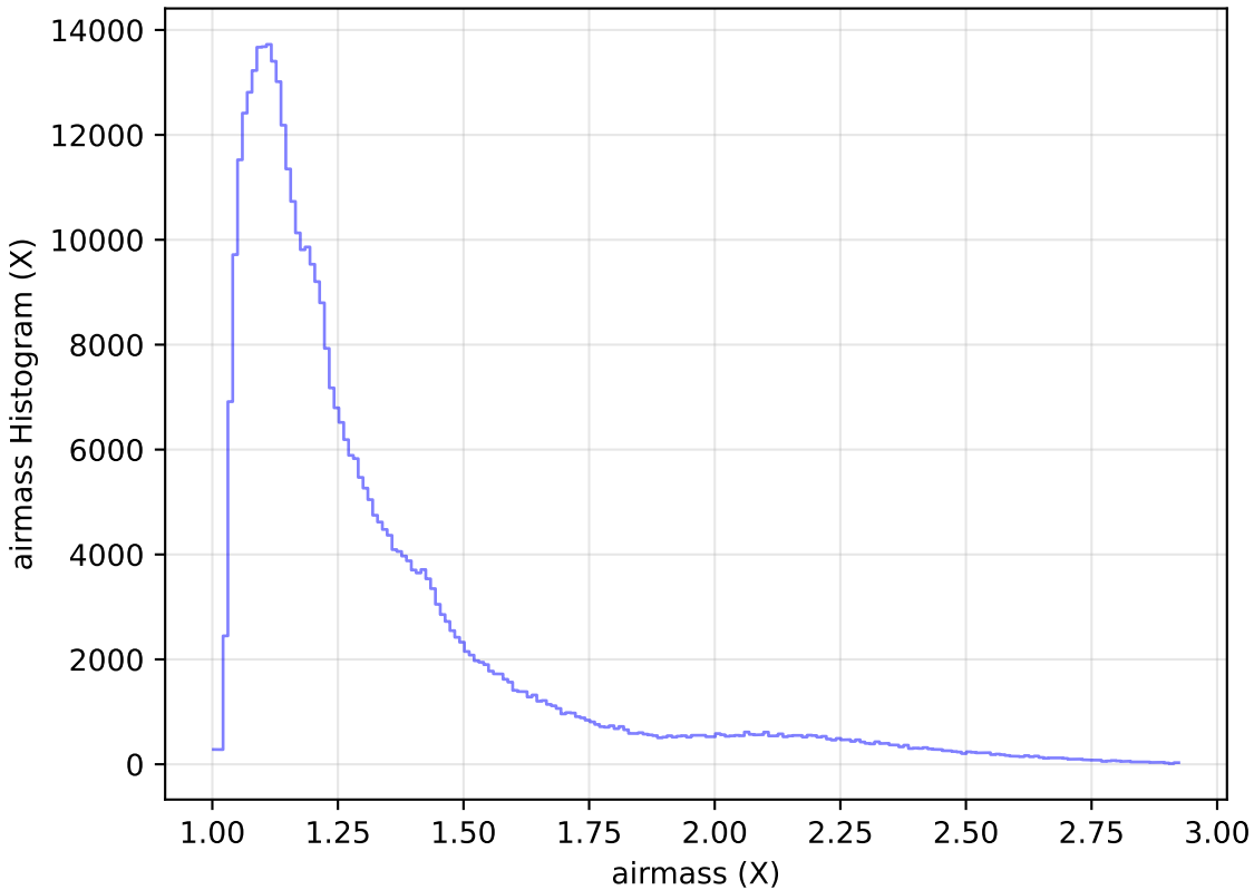
too_elab_r16_d3_griz_v3.4_10yrs WFD z band: airmass Histogram
