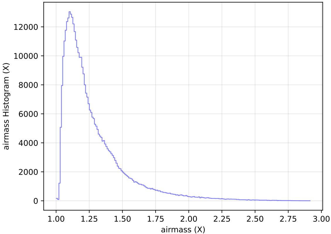
too_elab_r16_d3_griz_v3.4_10yrs WFD y band: airmass Histogram
