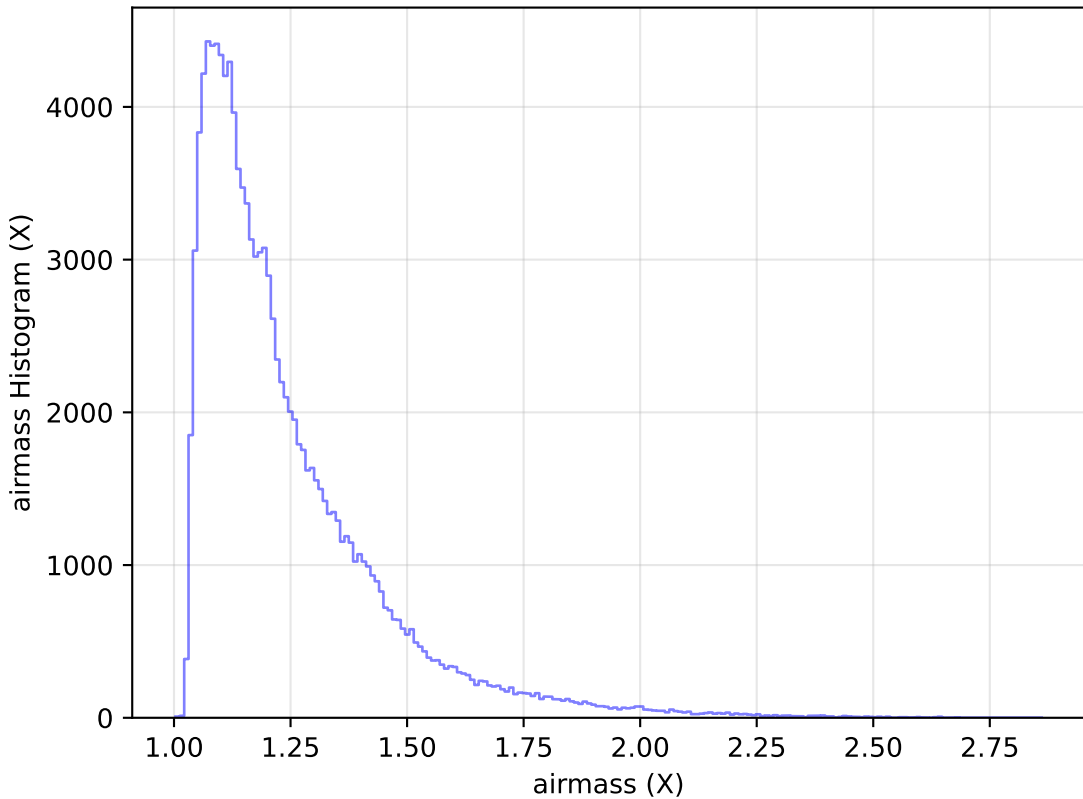
too_elab_r16_d3_griz_v3.4_10yrs WFD u band: airmass Histogram
