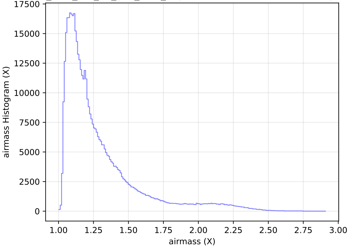
too_elab_r16_d3_griz_v3.4_10yrs WFD r band: airmass Histogram
