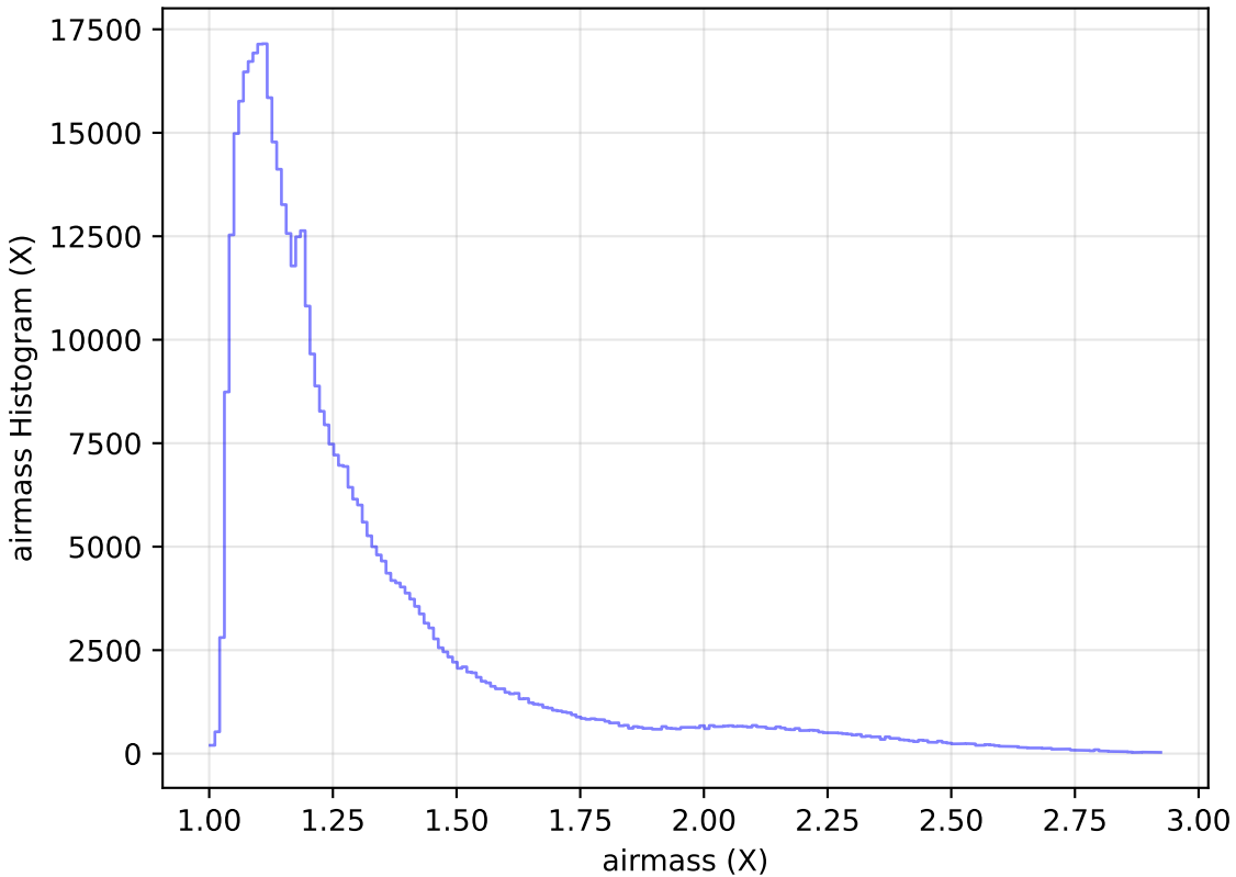
too_elab_r16_d3_griz_v3.4_10yrs WFD i band: airmass Histogram
