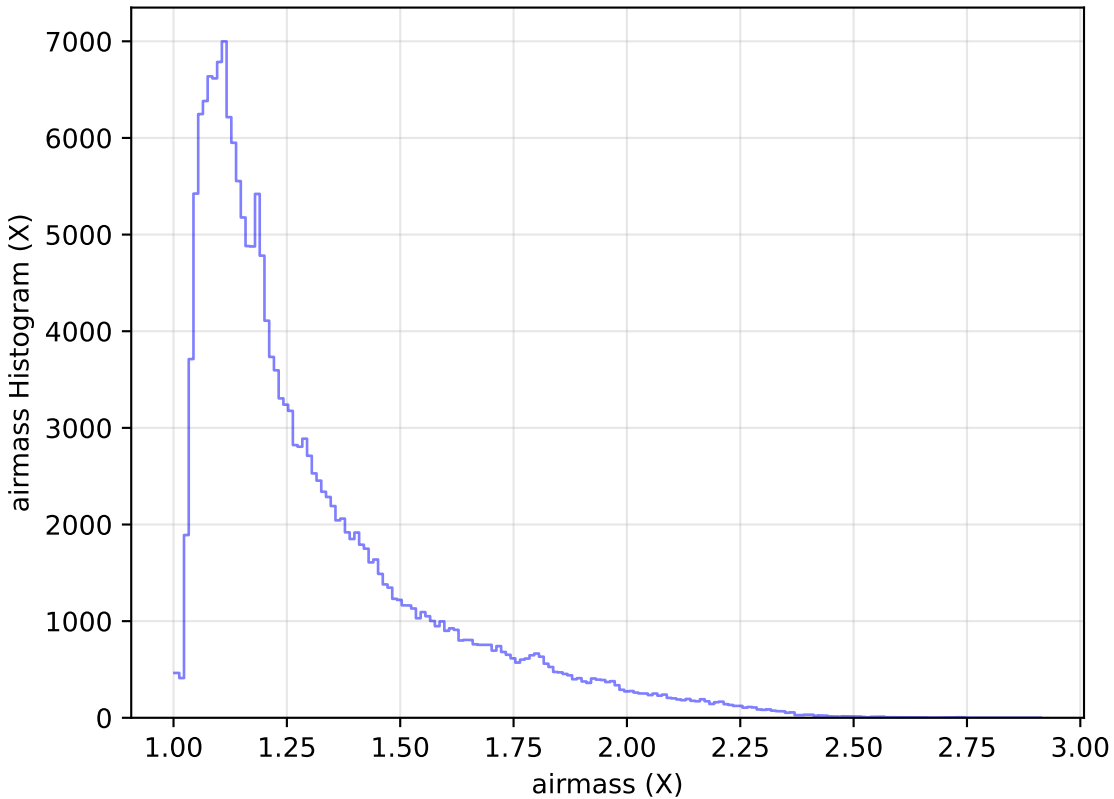
too_elab_r16_d3_griz_v3.4_10yrs WFD g band: airmass Histogram
