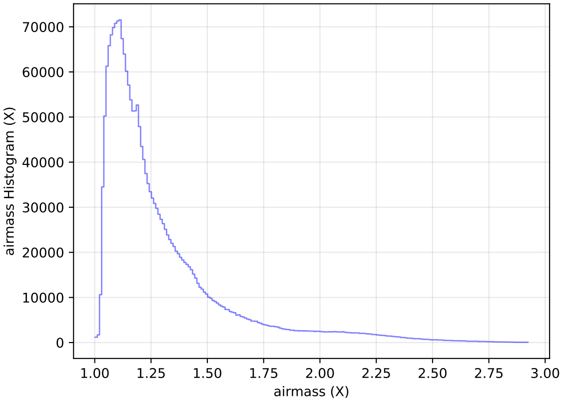
too_elab_r16_d3_griz_v3.4_10yrs WFD all bands: airmass Histogram
