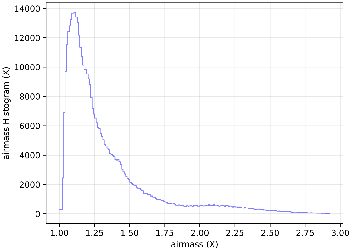
too_elab_r16_d3_griz_v3.4_10yrs All sky z band: airmass Histogram
