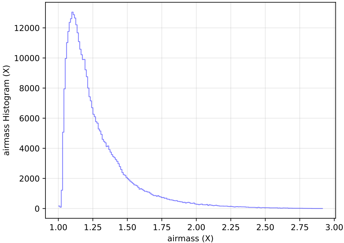
too_elab_r16_d3_griz_v3.4_10yrs All sky y band: airmass Histogram
