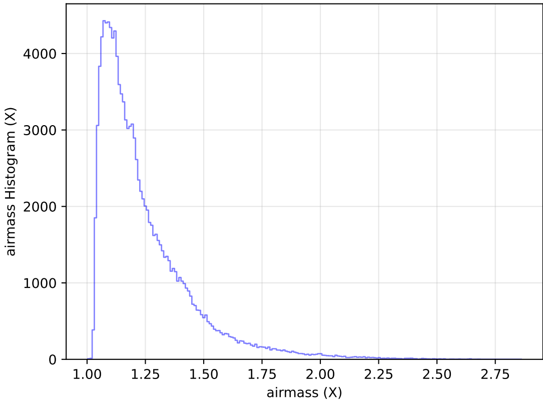
too_elab_r16_d3_griz_v3.4_10yrs All sky u band: airmass Histogram
