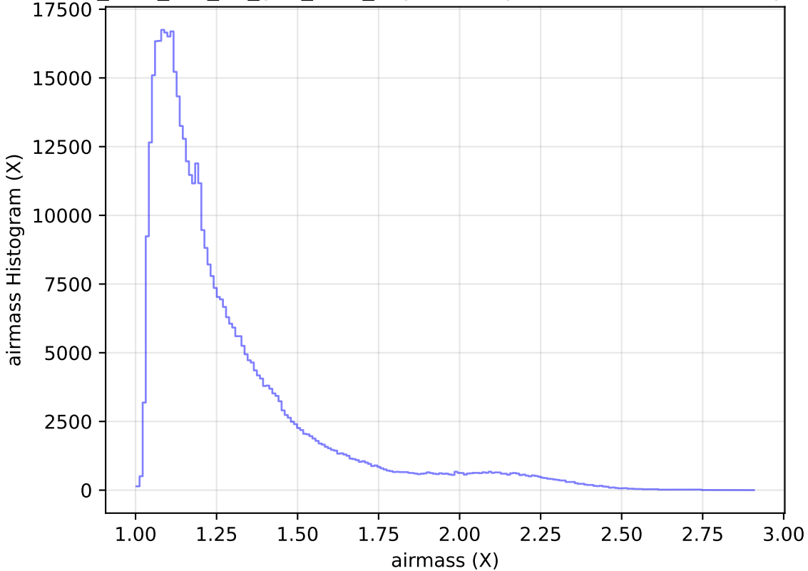
too_elab_r16_d3_griz_v3.4_10yrs All sky r band: airmass Histogram
