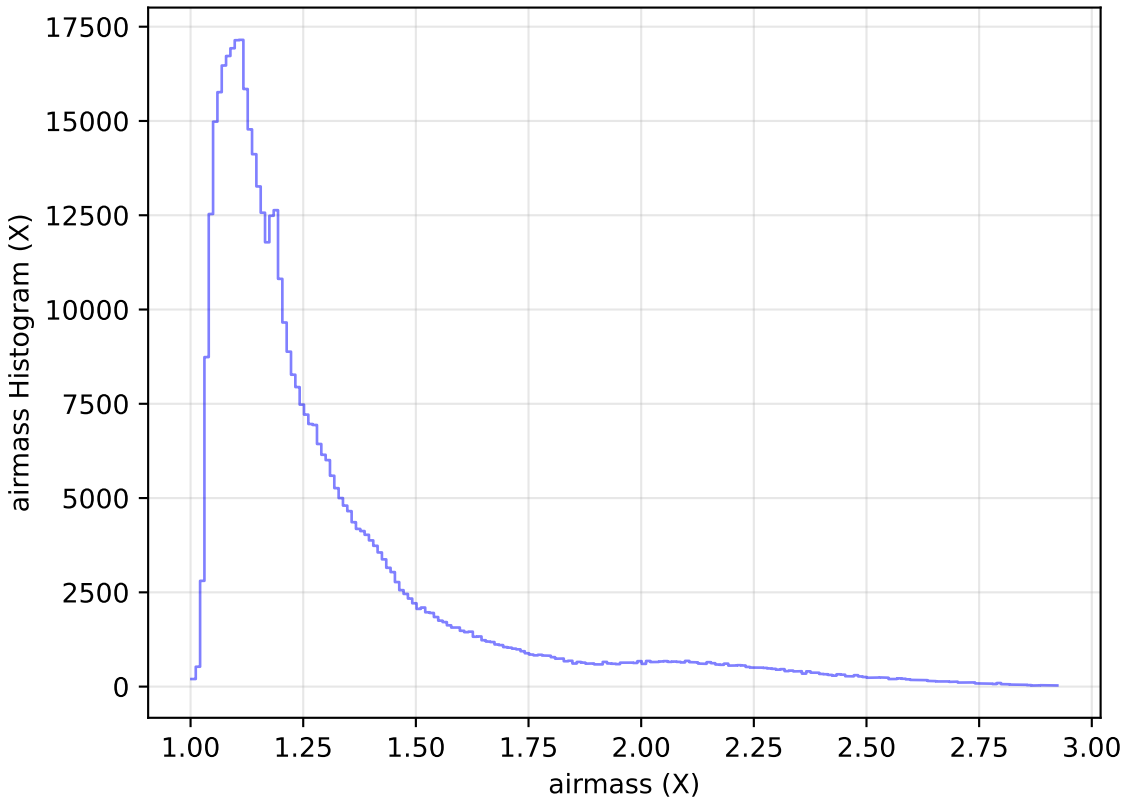
too_elab_r16_d3_griz_v3.4_10yrs All sky i band: airmass Histogram
