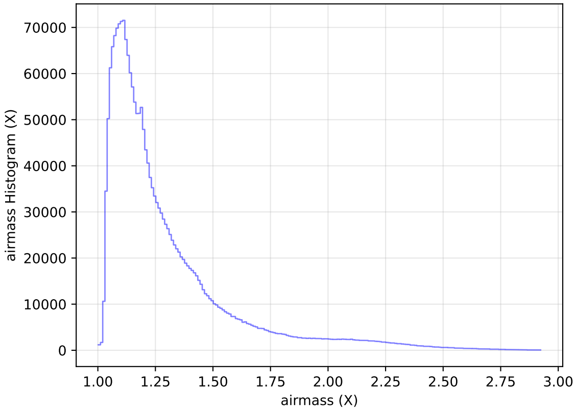
too_elab_r16_d3_griz_v3.4_10yrs All sky all bands: airmass Histogram
